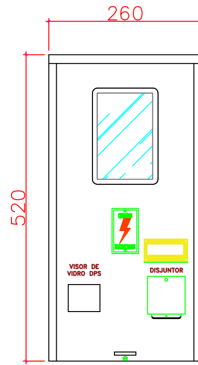
VISTA FRONTAL
